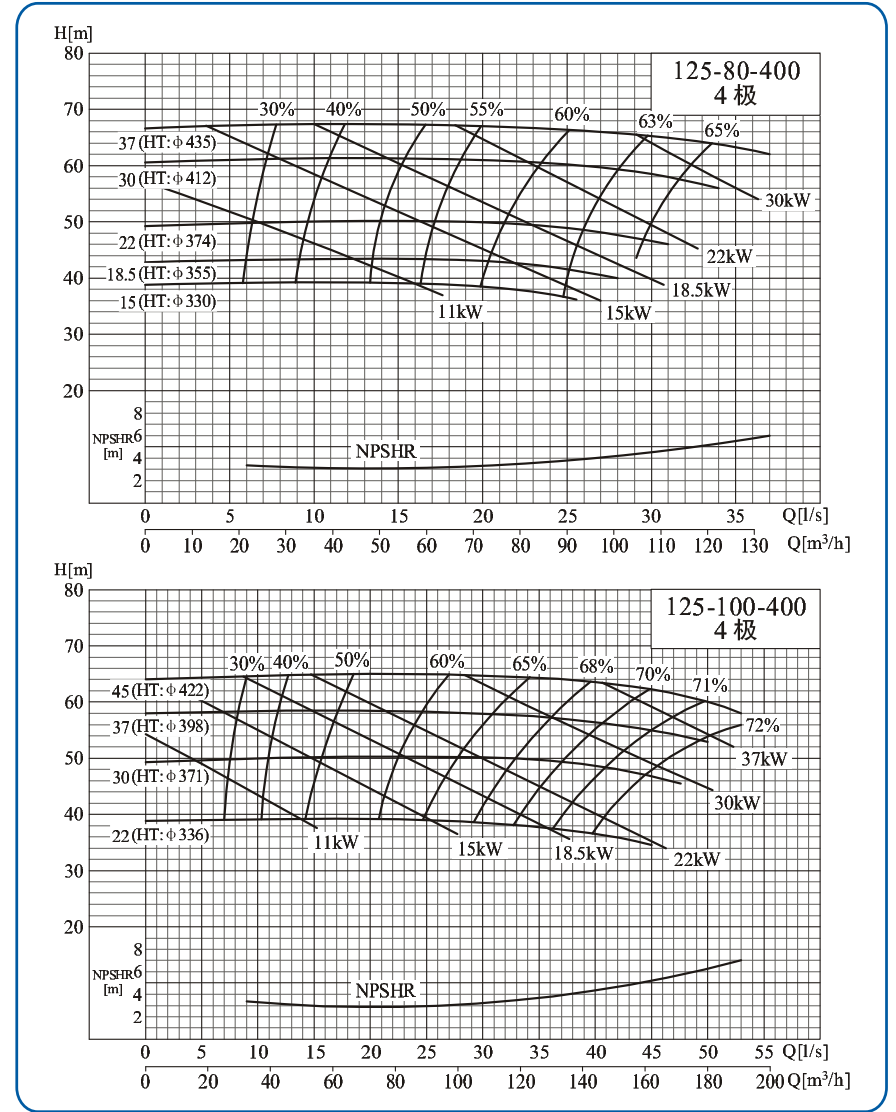
125-80-400/125-100-400
